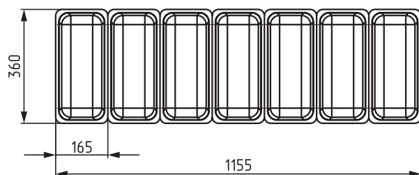
Displayed products gastronorm pans 360x165x120 – 7 pans
