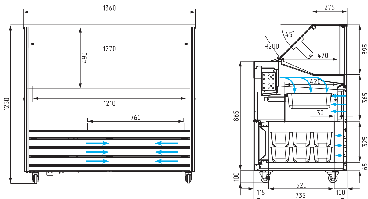
Layout of gastronorm pans in IC72SL1,3-1
