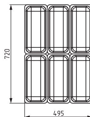
Storage section gastronorm pans 360x165x120 – 12 pans
